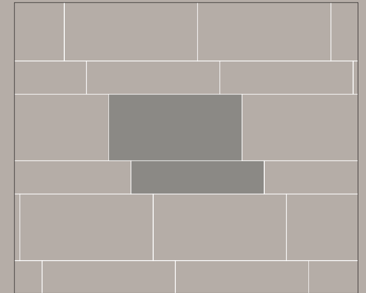
30x120 (12"x48") RT - 33,3% 60x120 (24"x48") RT - 66,6%
